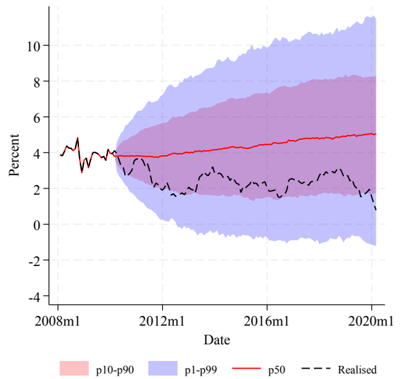
(b) 10-year yields forecasts from QE1
