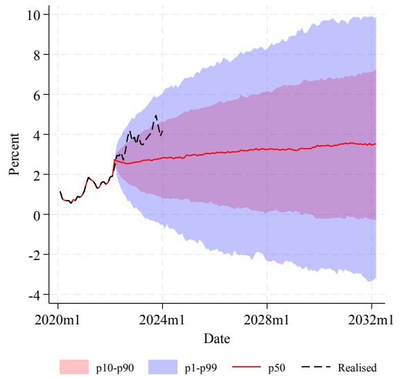
(d) 10-year yields forecasts from QE4
